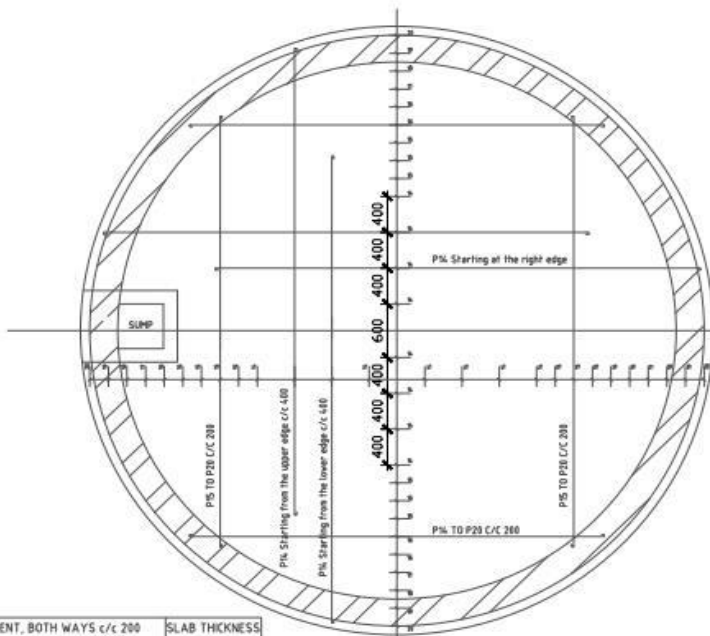
FLOOR REINFORCEMENT SCALE 1:50
