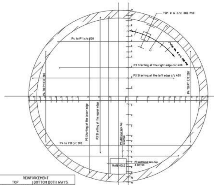
ROOF REINFORCEMENT SCALE 1:50
